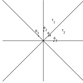
FIGURE 8. Topes \tau_1, \tau_2 for \Phi = (\phi_1, \phi_2, \phi_3 = \frac{1}{2}(\phi_2 - \phi_1), \phi_4 = \frac{1}{2}(\phi_1 + \phi_2)) .
