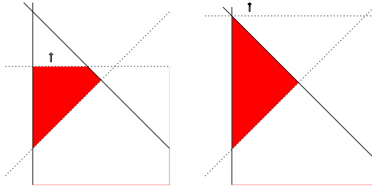
FIGURE 11. \lambda_1 > -\lambda_2 > 0 , (tope (\phi_1, -\phi_3) ), then \lambda_1 = -\lambda_2 > 0 , (wall (-\phi_3) ).
