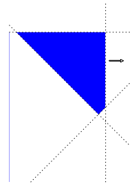
FIGURE 13. \lambda_1 < \lambda_2 < 0 , (tope (-\phi_2, -\phi_4) ). The polygon is now the interior of the opposite of the initial tetragon of Fig. 9, cf [20].
