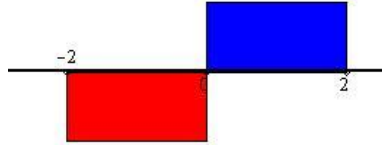
FIGURE 1. In blue for b = (0, 2) , q(b) = [0, 2] , in red for b = (0, -2) , A(b) = (-1) times ] - 2, 0[
