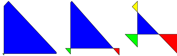
FIGURE 17. From left to right, \lambda crosses three walls, one at a time. The new triangles have multiplicity -1 .
