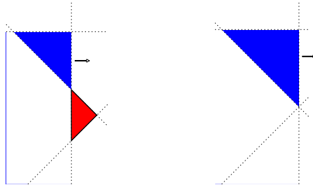
FIGURE 12. -\lambda_2 > \lambda_1 > 0 , (tope (-\phi_3, -\phi_2) ), then -\lambda_2 > 0 = \lambda_1 , (wall -\phi_2 ).
