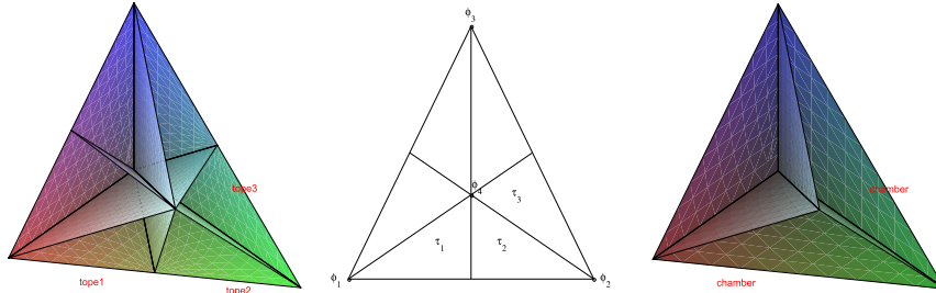
FIGURE 6. Left, topes for \Phi = (\phi_1, \phi_2, \phi_3, \phi_1 + \phi_2 + \phi_3) . Right, chambers.
