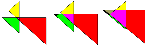
FIGURE 18. \lambda crosses three more walls. The polytope colored in magenta has multiplicity -2 .
