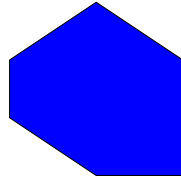
FIGURE 16. At the beginning \lambda = (200, -100, 200, 400) is in the ample cone. The partition polytope is an hexagon.
